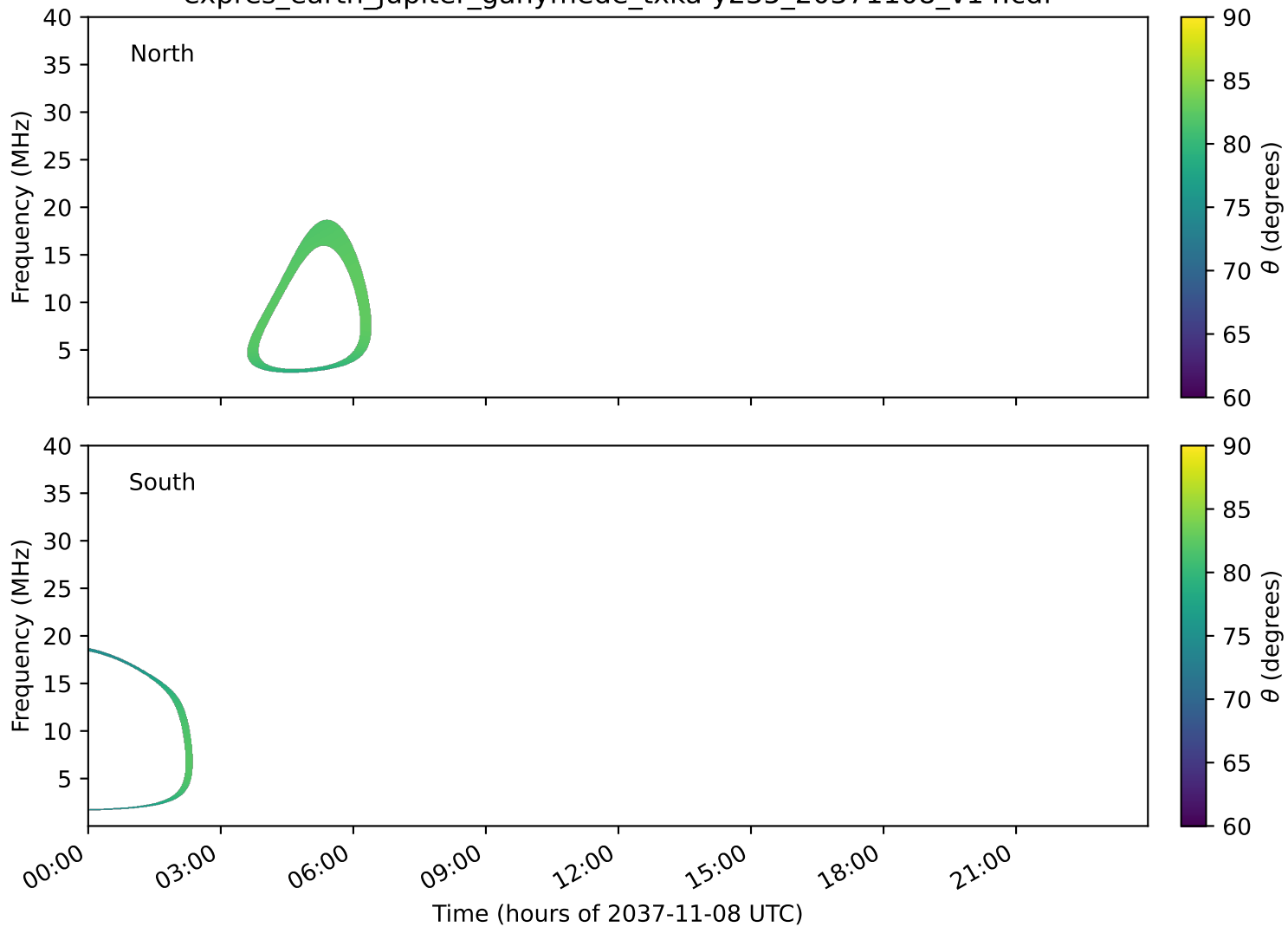
expres_earth_jupiter_ganymede_txka-y235_20371108_v14.cdf
