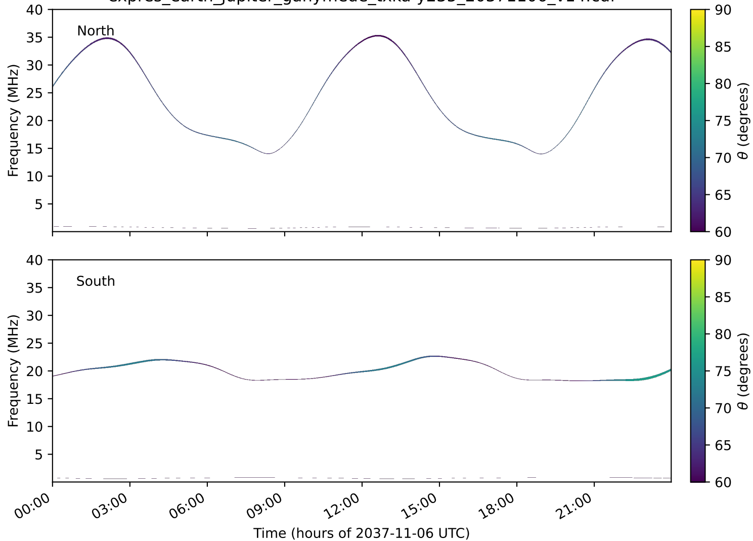
expres_earth_jupiter_ganymede_txka-y235_20371106_v14.cdf
