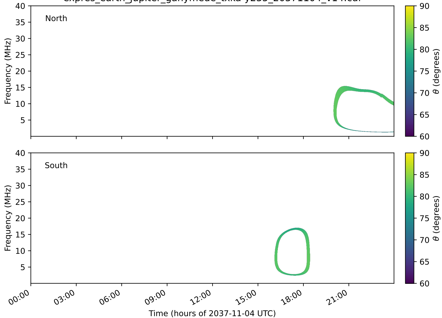
expres_earth_jupiter_ganymede_txka-y235_20371104_v14.cdf
