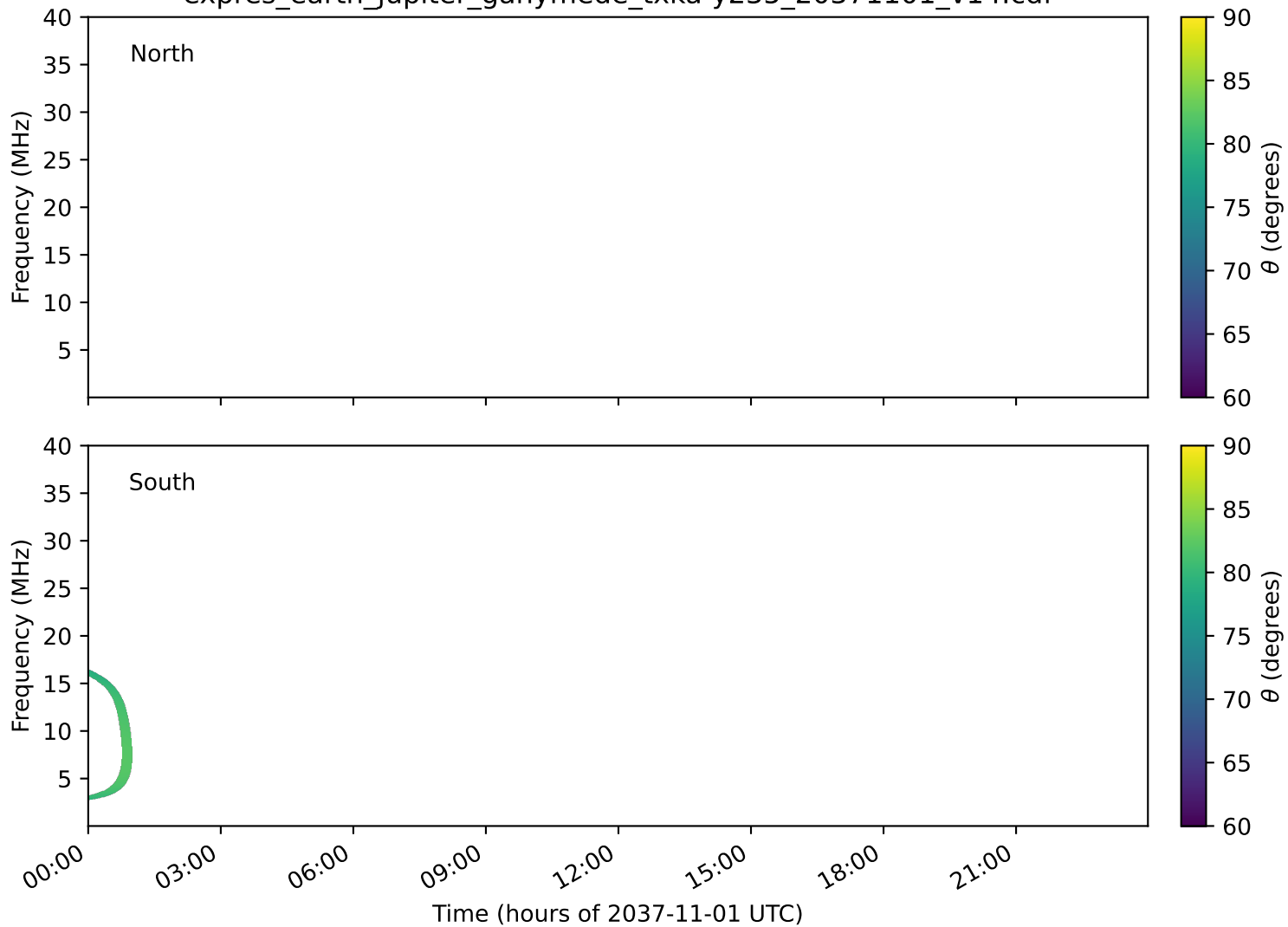
expres_earth_jupiter_ganymede_txka-y235_20371101_v14.cdf
