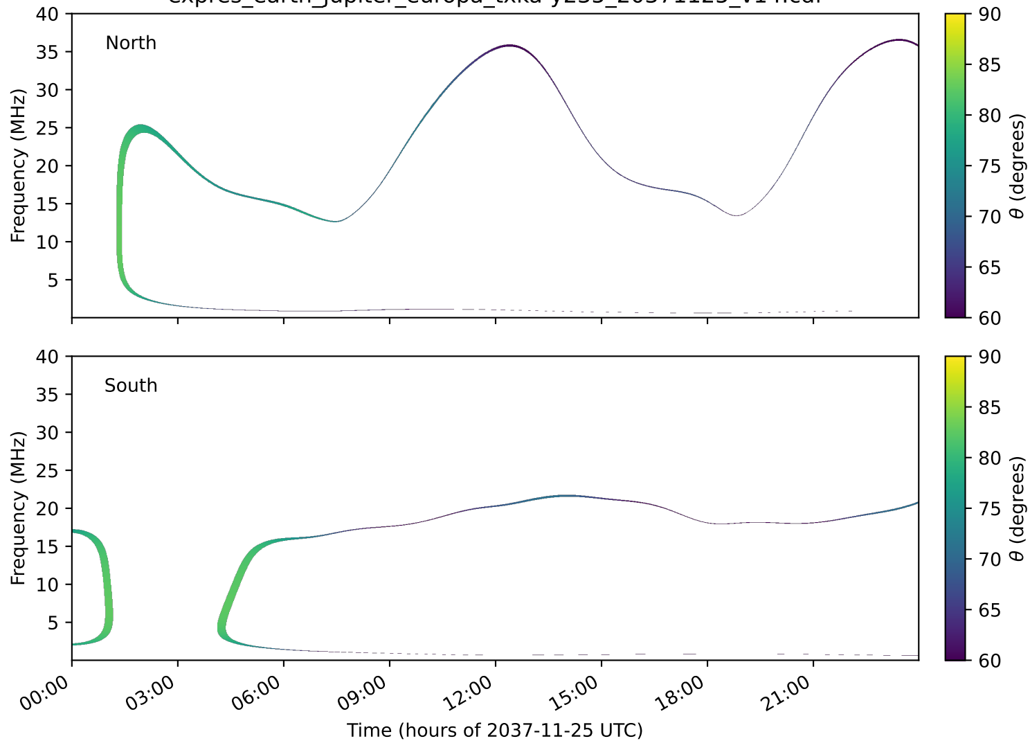
expres_earth_jupiter_europa_txka-y235_20371125_v14.cdf
