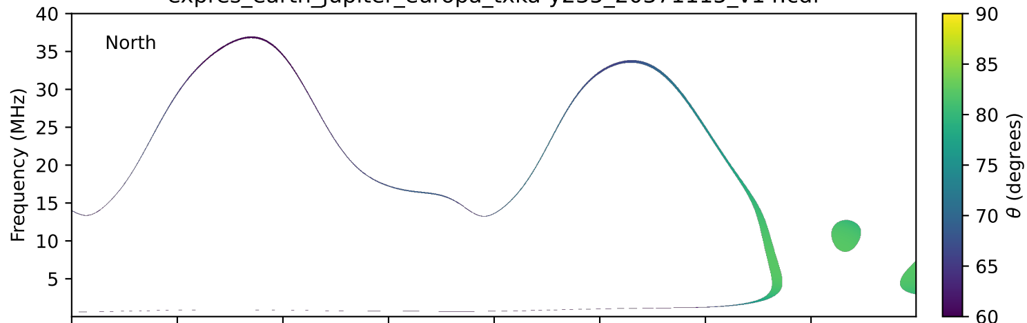
expres_earth_jupiter_europa_txka-y235_20371115_v14.cdf
