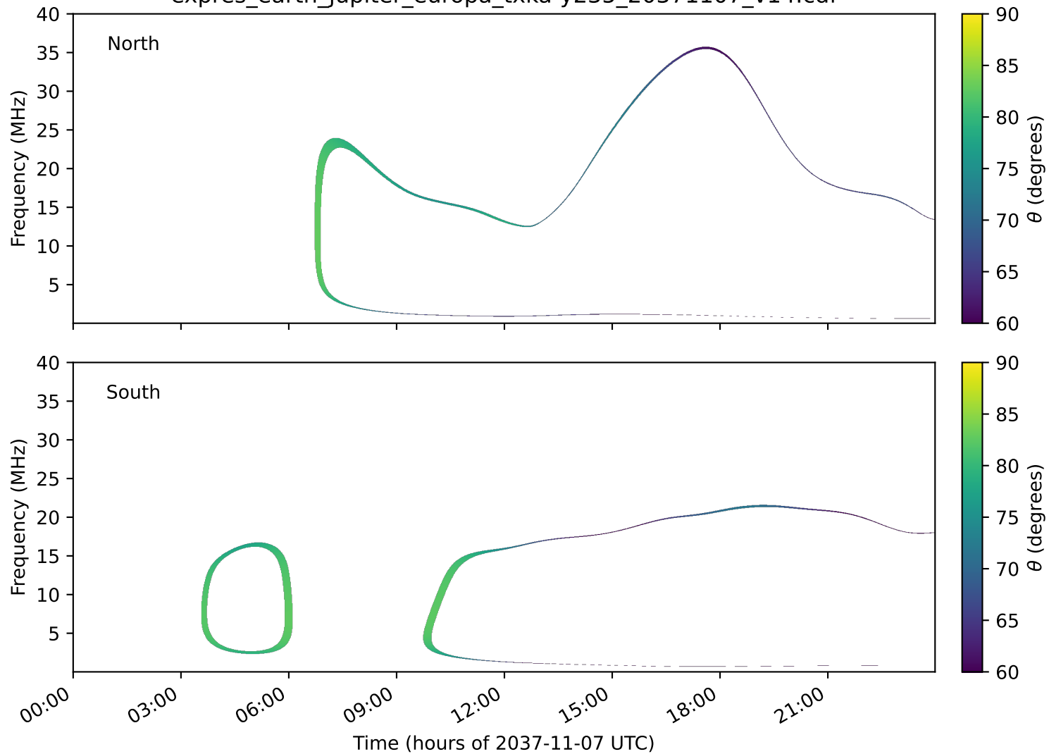
expres_earth_jupiter_europa_txka-y235_20371107_v14.cdf
