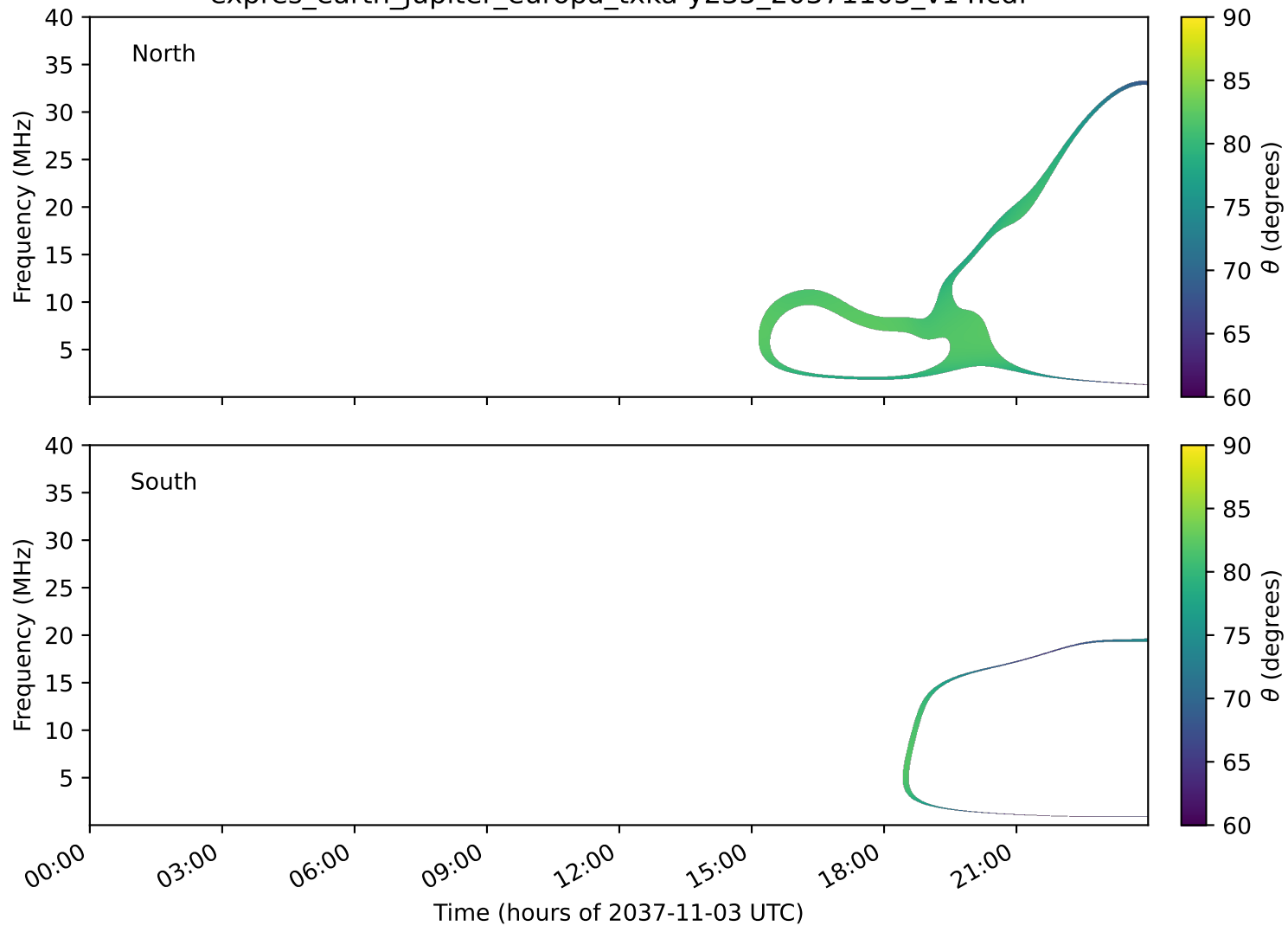
expres_earth_jupiter_europa_txka-y235_20371103_v14.cdf
