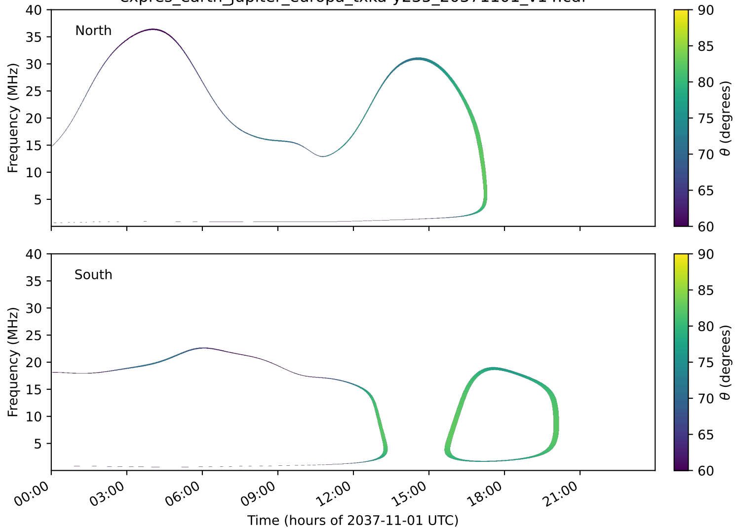
expres_earth_jupiter_europa_txka-y235_20371101_v14.cdf
