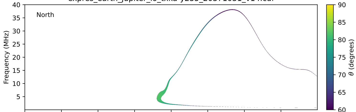
expres_earth_jupiter_io_txka-y235_20371031_v14.cdf
