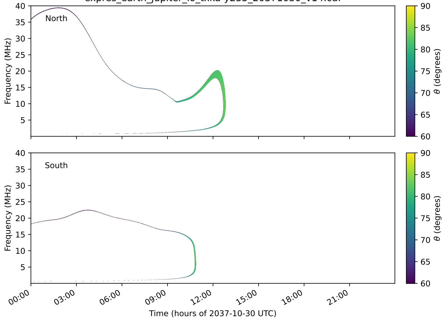
expres_earth_jupiter_io_txka-y235_20371030_v14.cdf
