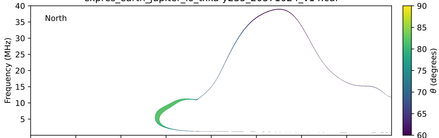
expres_earth_jupiter_io_txka-y235_20371024_v14.cdf
