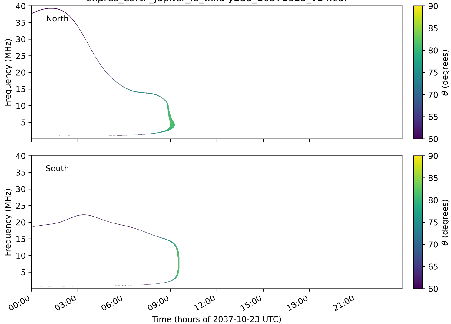
expres_earth_jupiter_io_txka-y235_20371023_v14.cdf
