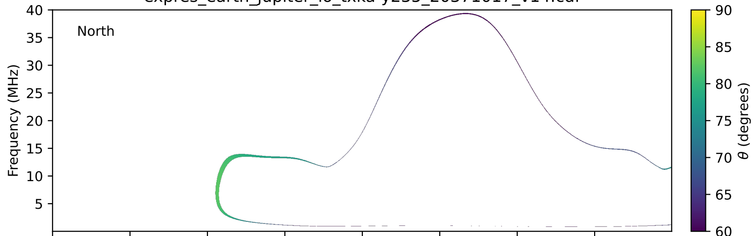
expres_earth_jupiter_io_txka-y235_20371017_v14.cdf
