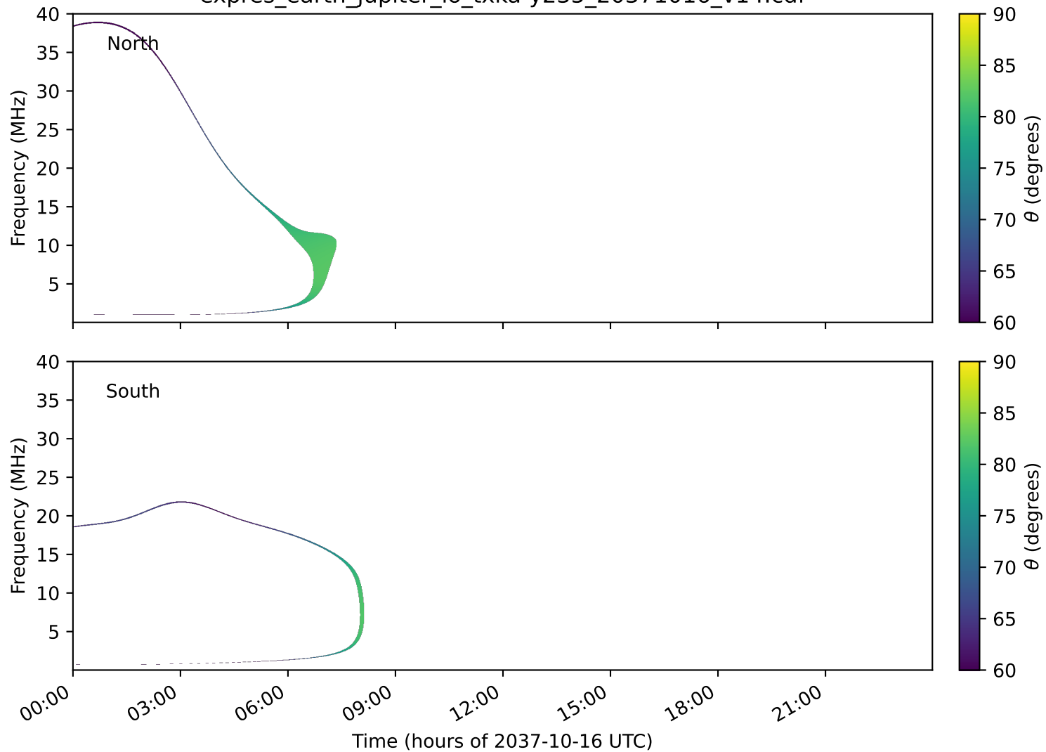
expres_earth_jupiter_io_txka-y235_20371016_v14.cdf
