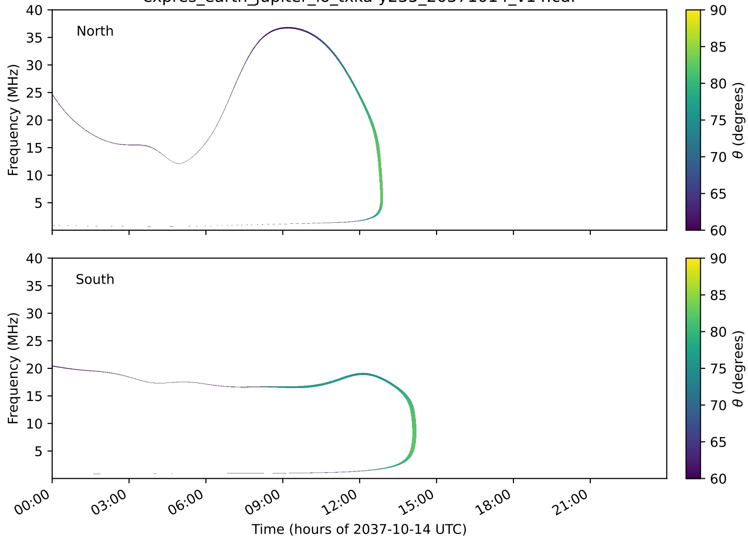
expres_earth_jupiter_io_txka-y235_20371014_v14.cdf
