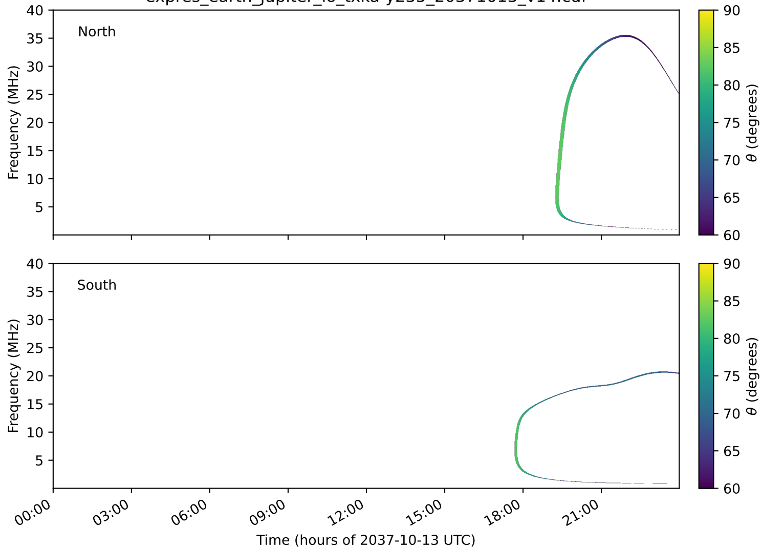
expres_earth_jupiter_io_txka-y235_20371013_v14.cdf
