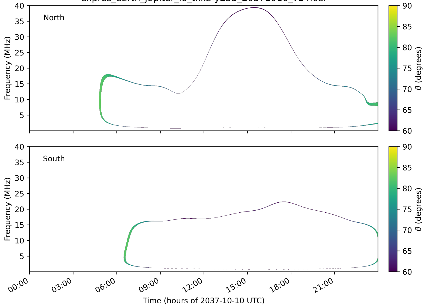
expres_earth_jupiter_io_txka-y235_20371010_v14.cdf
