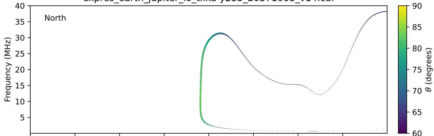
expres_earth_jupiter_io_txka-y235_20371008_v14.cdf
