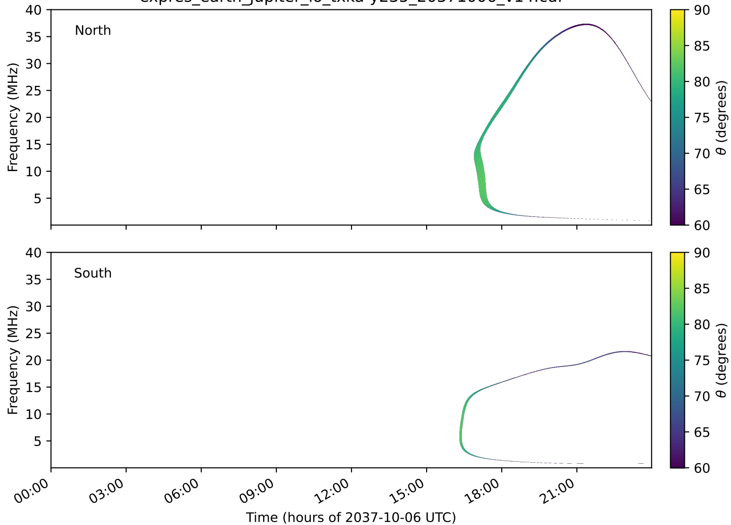
expres_earth_jupiter_io_txka-y235_20371006_v14.cdf
