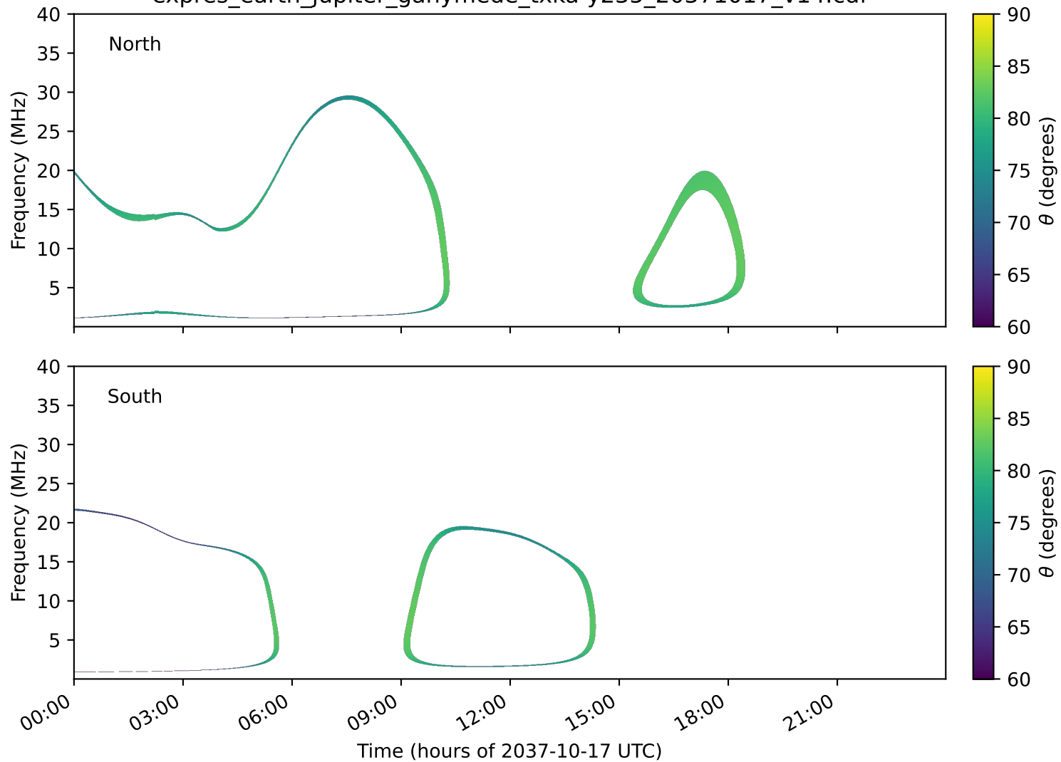
expres_earth_jupiter_ganymede_txka-y235_20371017_v14.cdf
