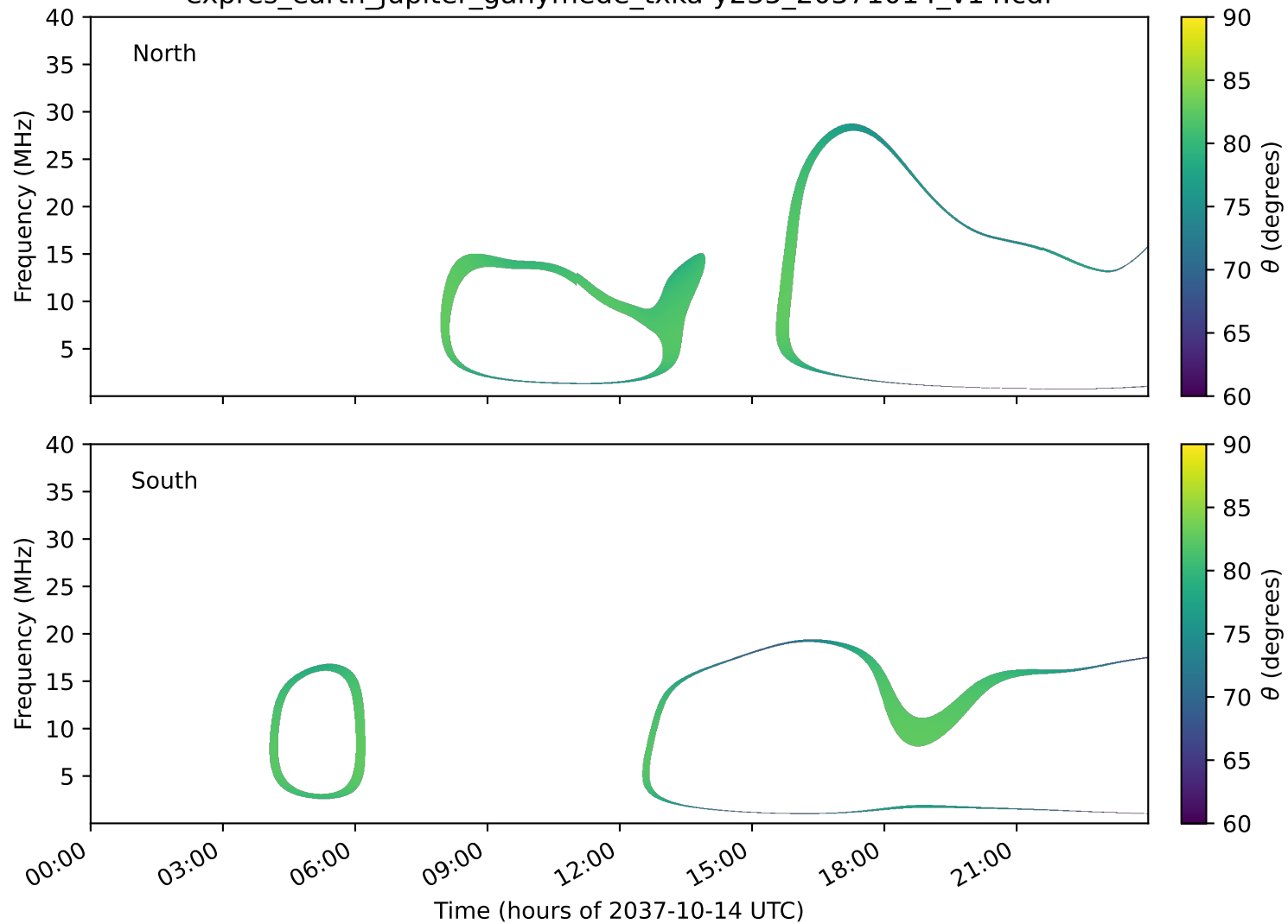
expres_earth_jupiter_ganymede_txka-y235_20371014_v14.cdf
