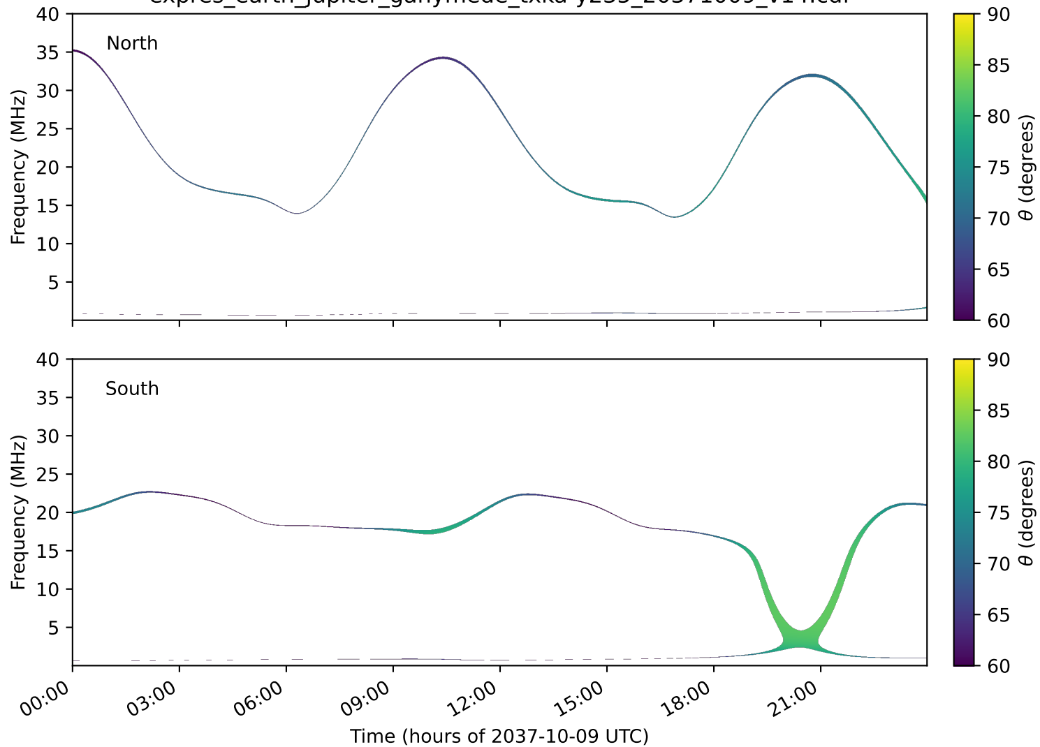
expres_earth_jupiter_ganymede_txka-y235_20371009_v14.cdf
