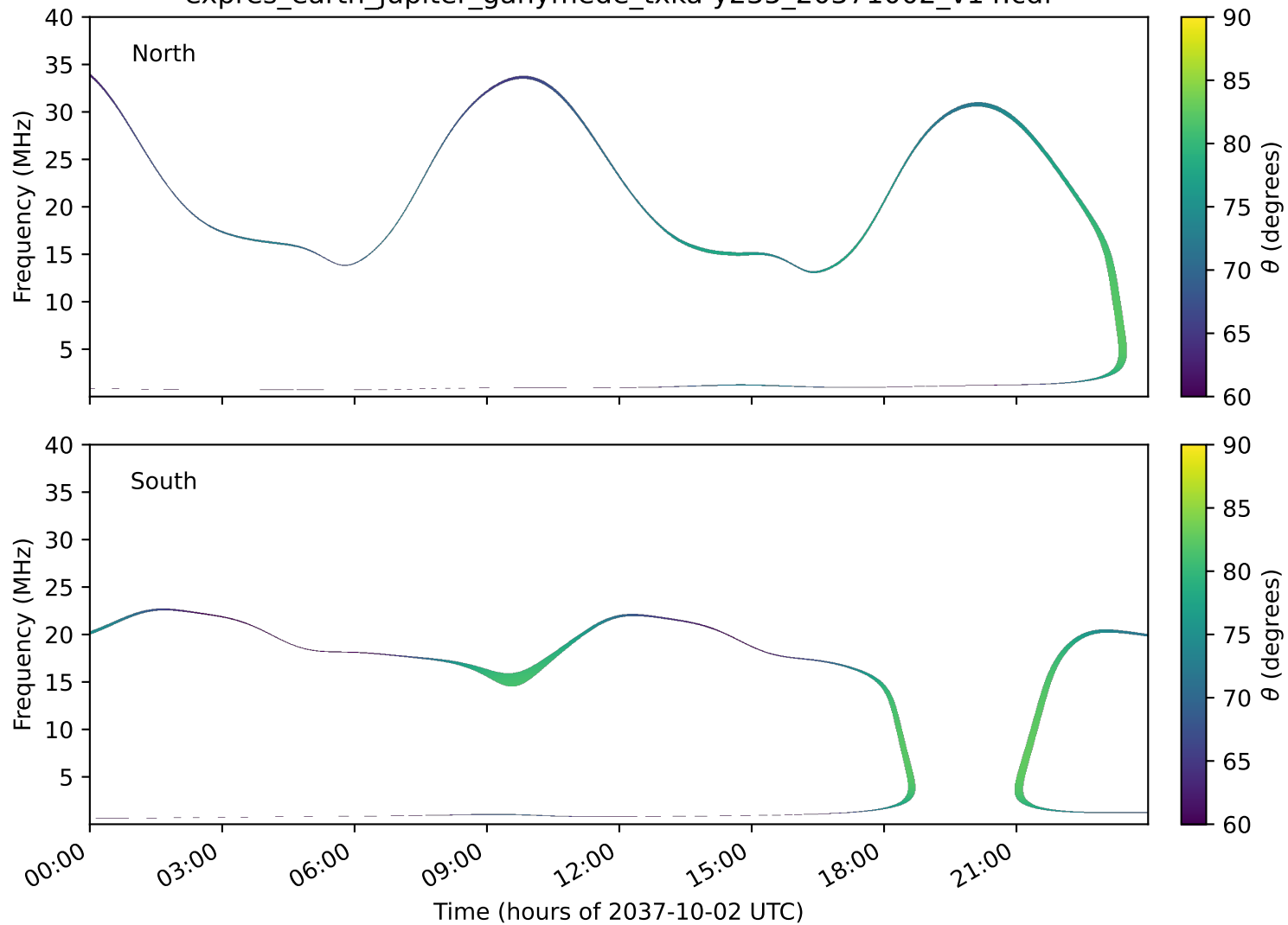
expres_earth_jupiter_ganymede_txka-y235_20371002_v14.cdf
