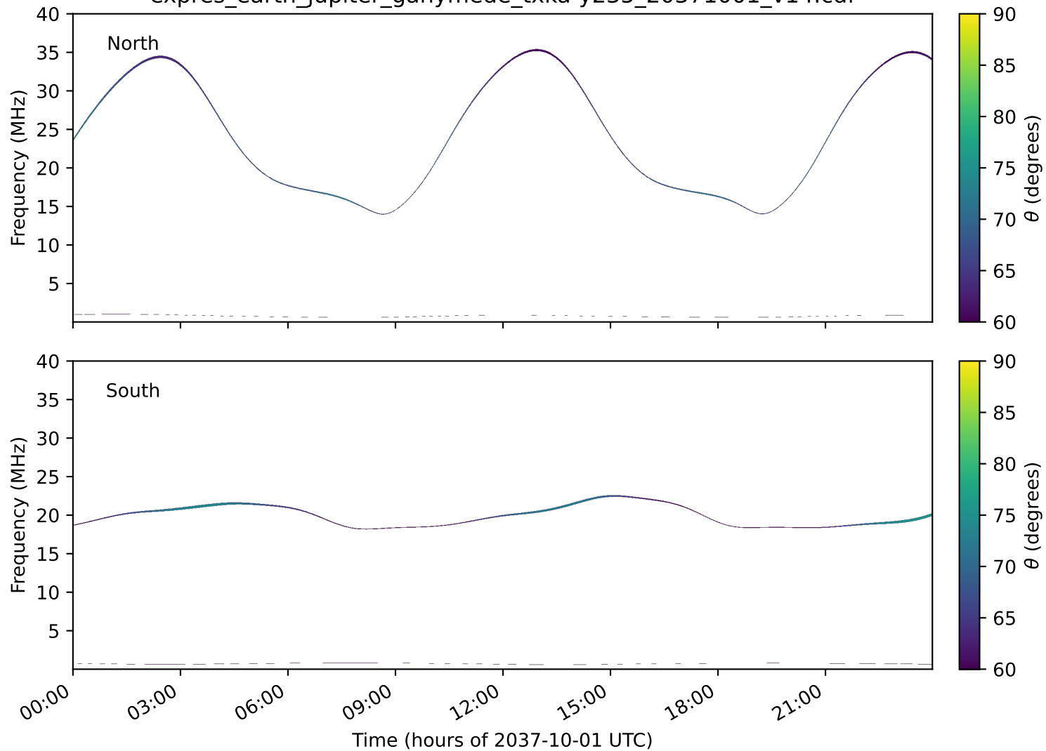
expres_earth_jupiter_ganymede_txka-y235_20371001_v14.cdf
