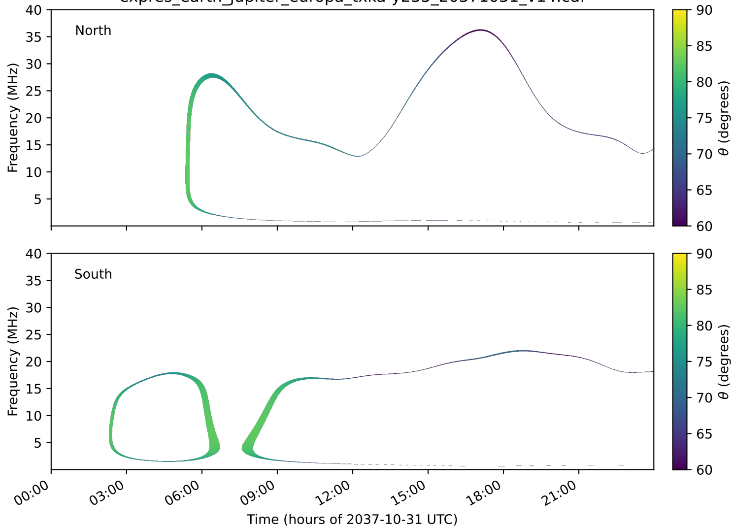
expres_earth_jupiter_europa_txka-y235_20371031_v14.cdf
