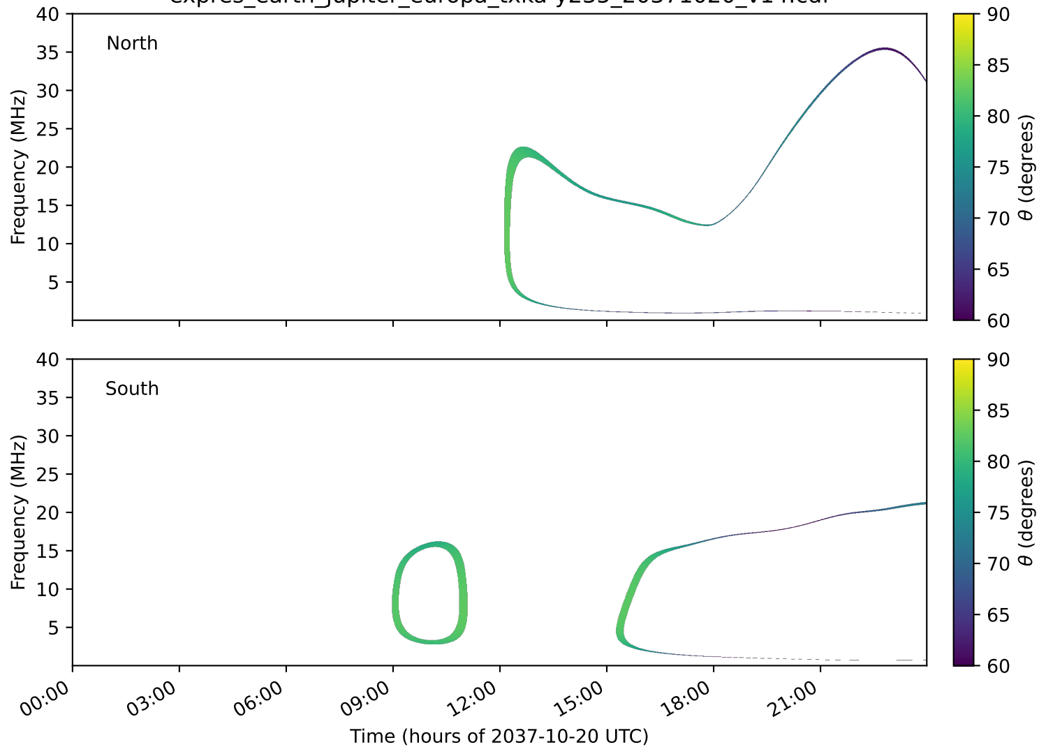
expres_earth_jupiter_europa_txka-y235_20371020_v14.cdf
