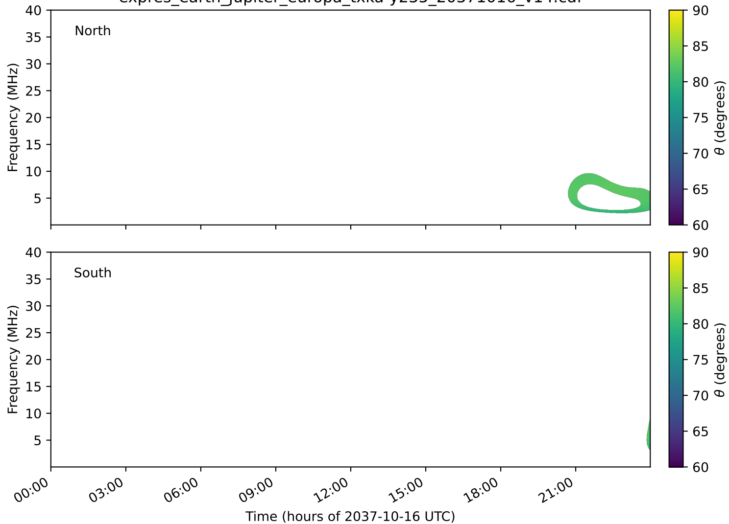
expres_earth_jupiter_europa_txka-y235_20371016_v14.cdf
