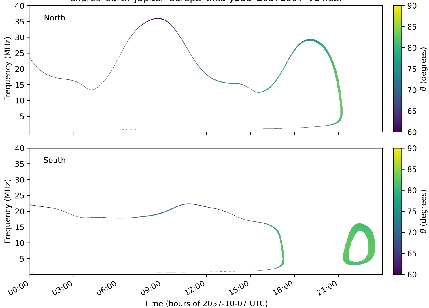
expres_earth_jupiter_europa_txka-y235_20371007_v14.cdf
