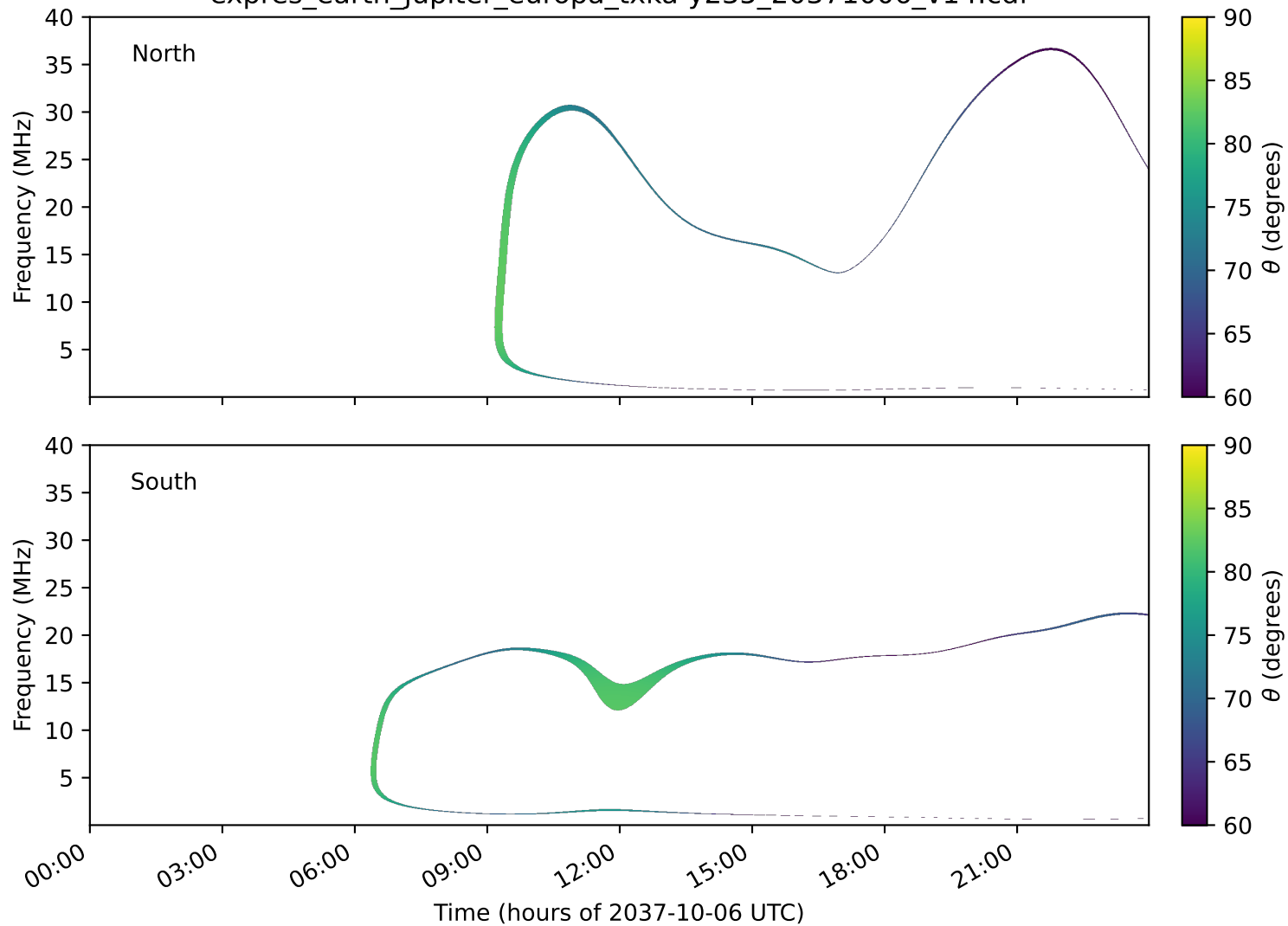
expres_earth_jupiter_europa_txka-y235_20371006_v14.cdf
