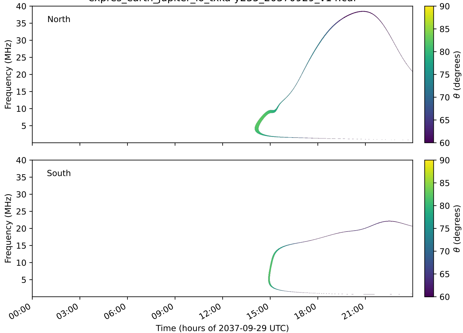
expres_earth_jupiter_io_txka-y235_20370929_v14.cdf
