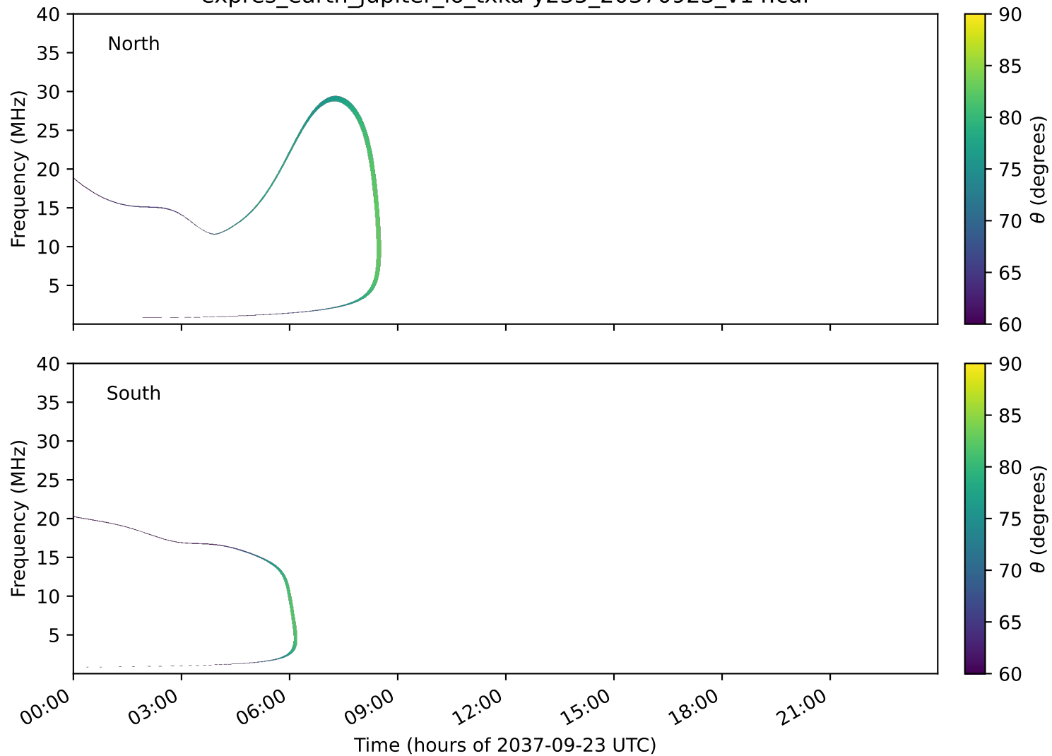
expres_earth_jupiter_io_txka-y235_20370923_v14.cdf
