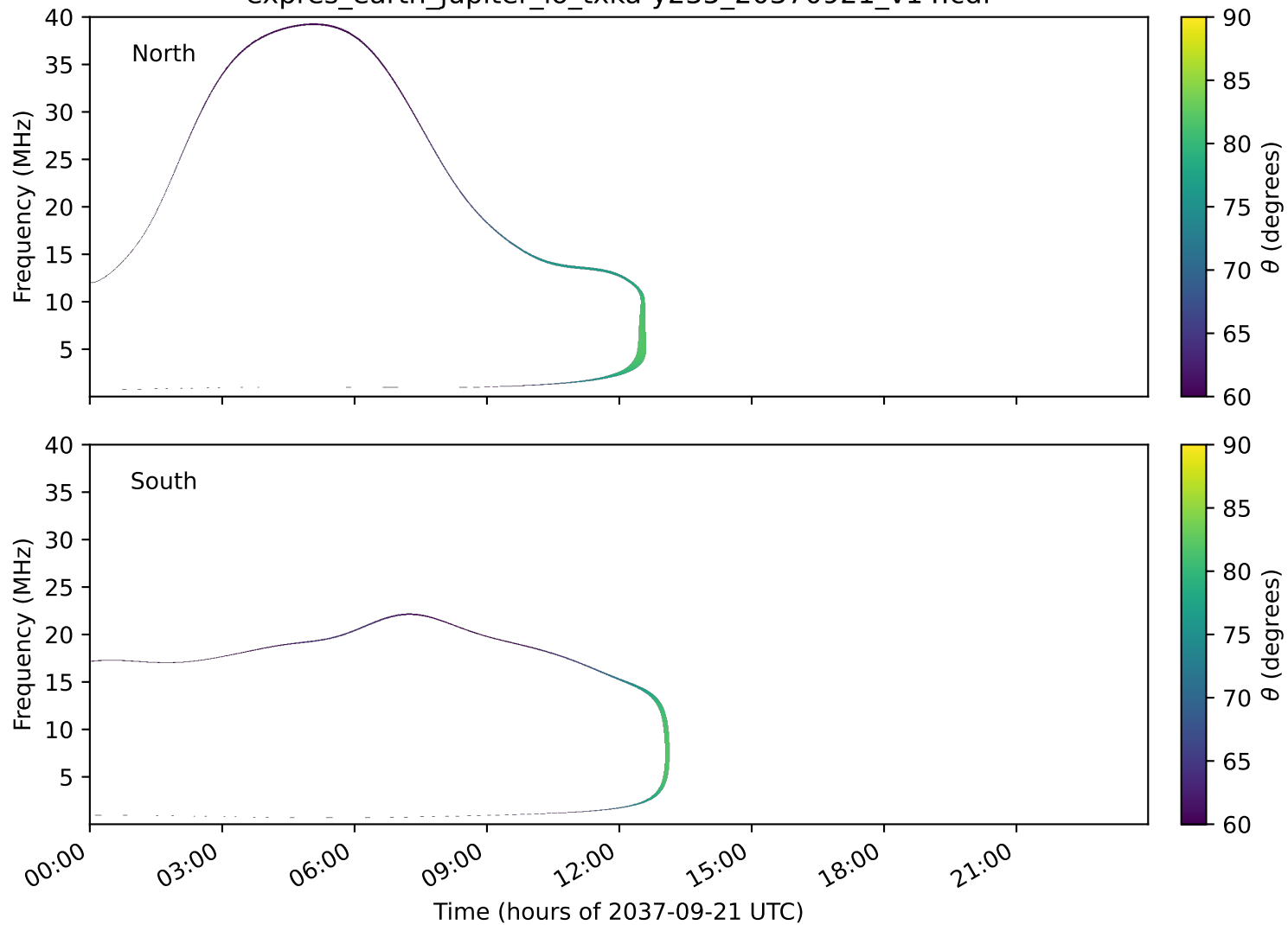
expres_earth_jupiter_io_txka-y235_20370921_v14.cdf
