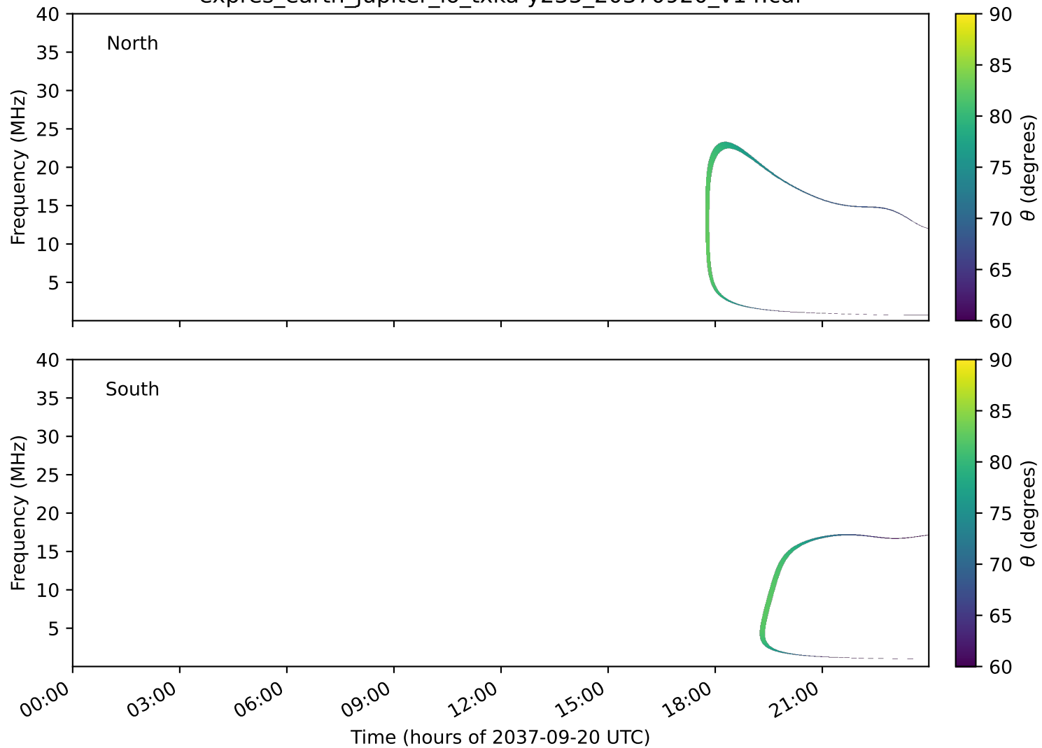
expres_earth_jupiter_io_txka-y235_20370920_v14.cdf
