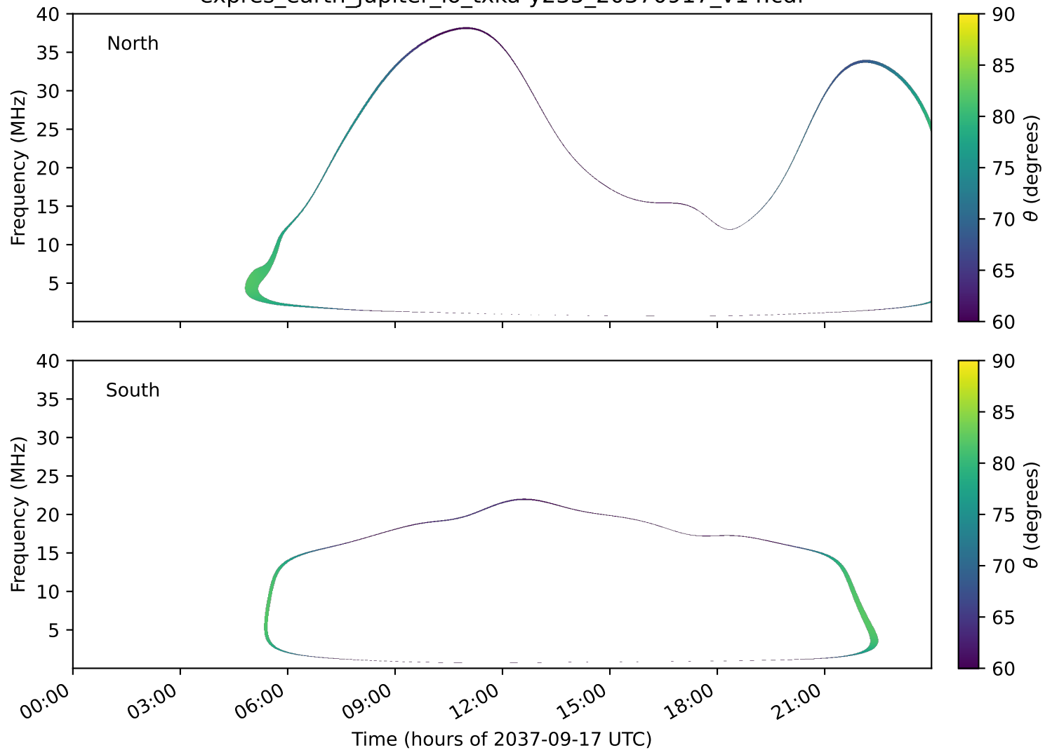
expres_earth_jupiter_io_txka-y235_20370917_v14.cdf
