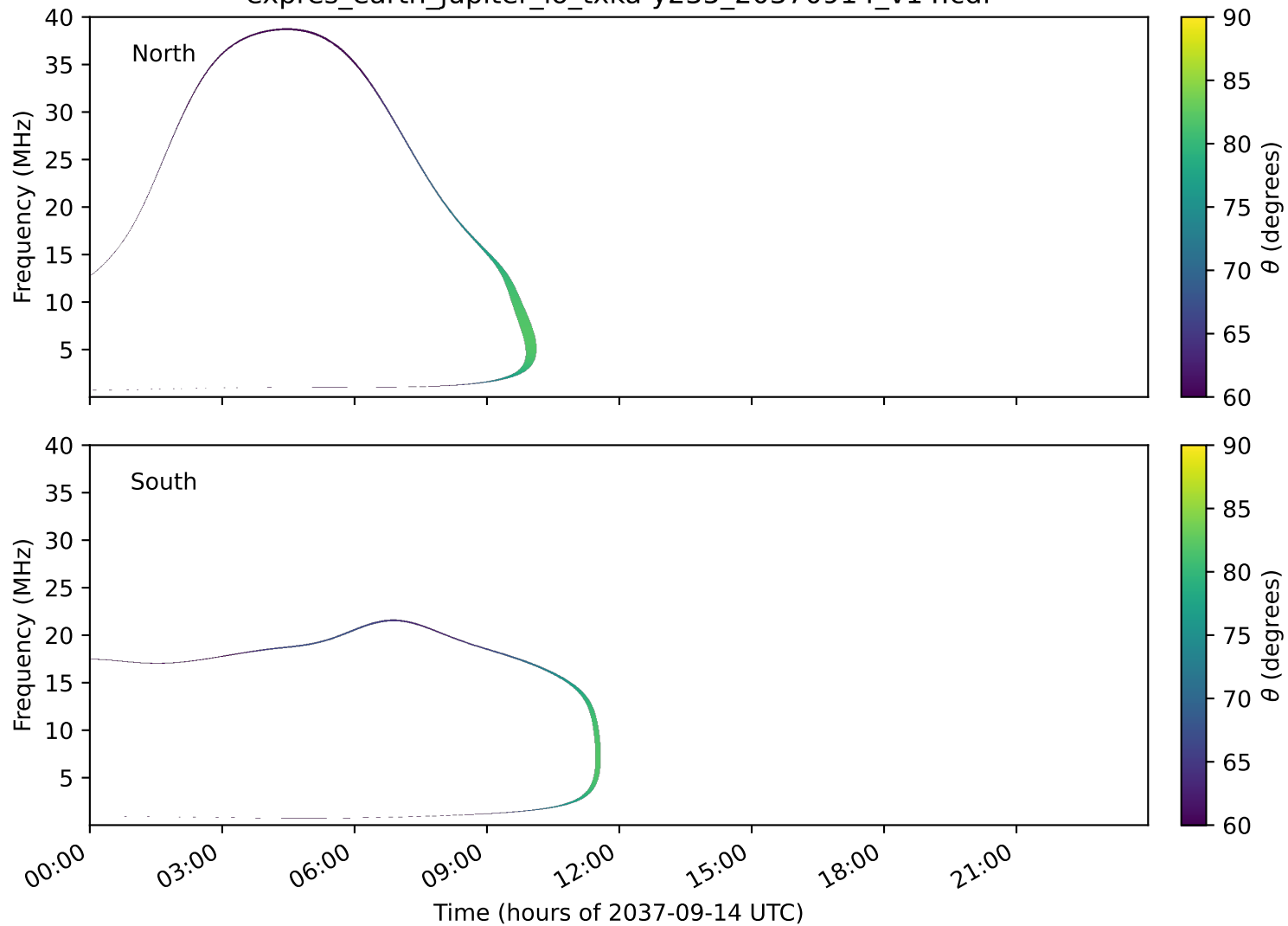
expres_earth_jupiter_io_txka-y235_20370914_v14.cdf
