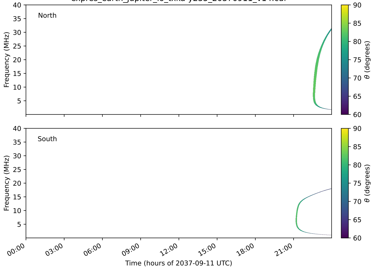
expres_earth_jupiter_io_txka-y235_20370911_v14.cdf
