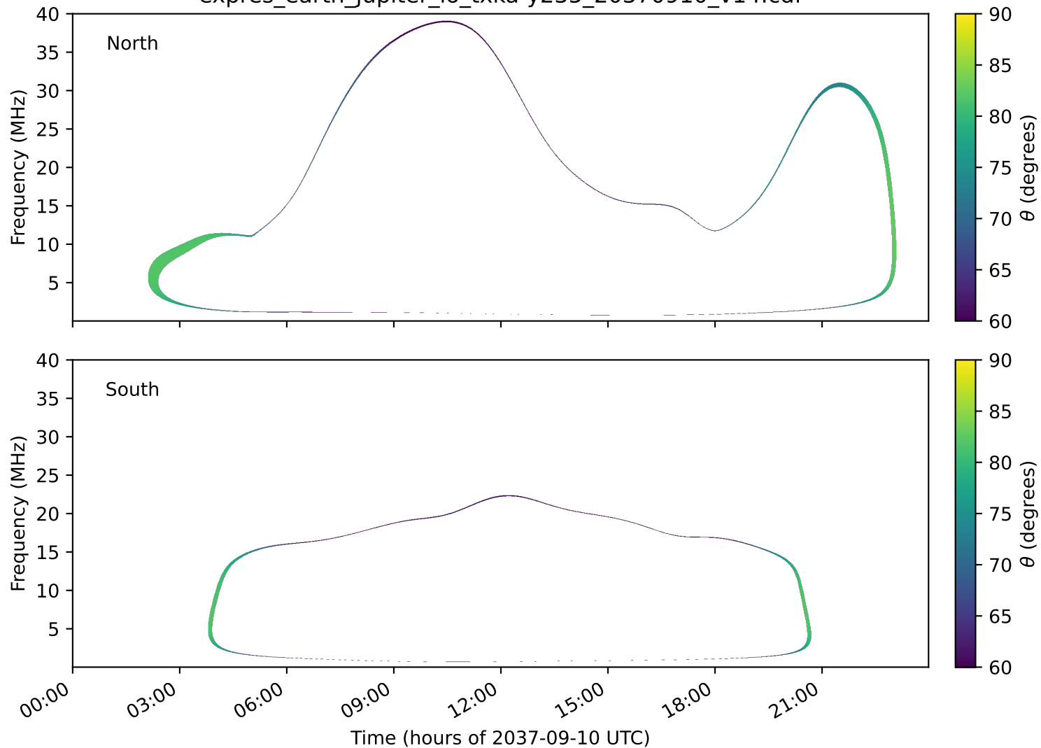
expres_earth_jupiter_io_txka-y235_20370910_v14.cdf
