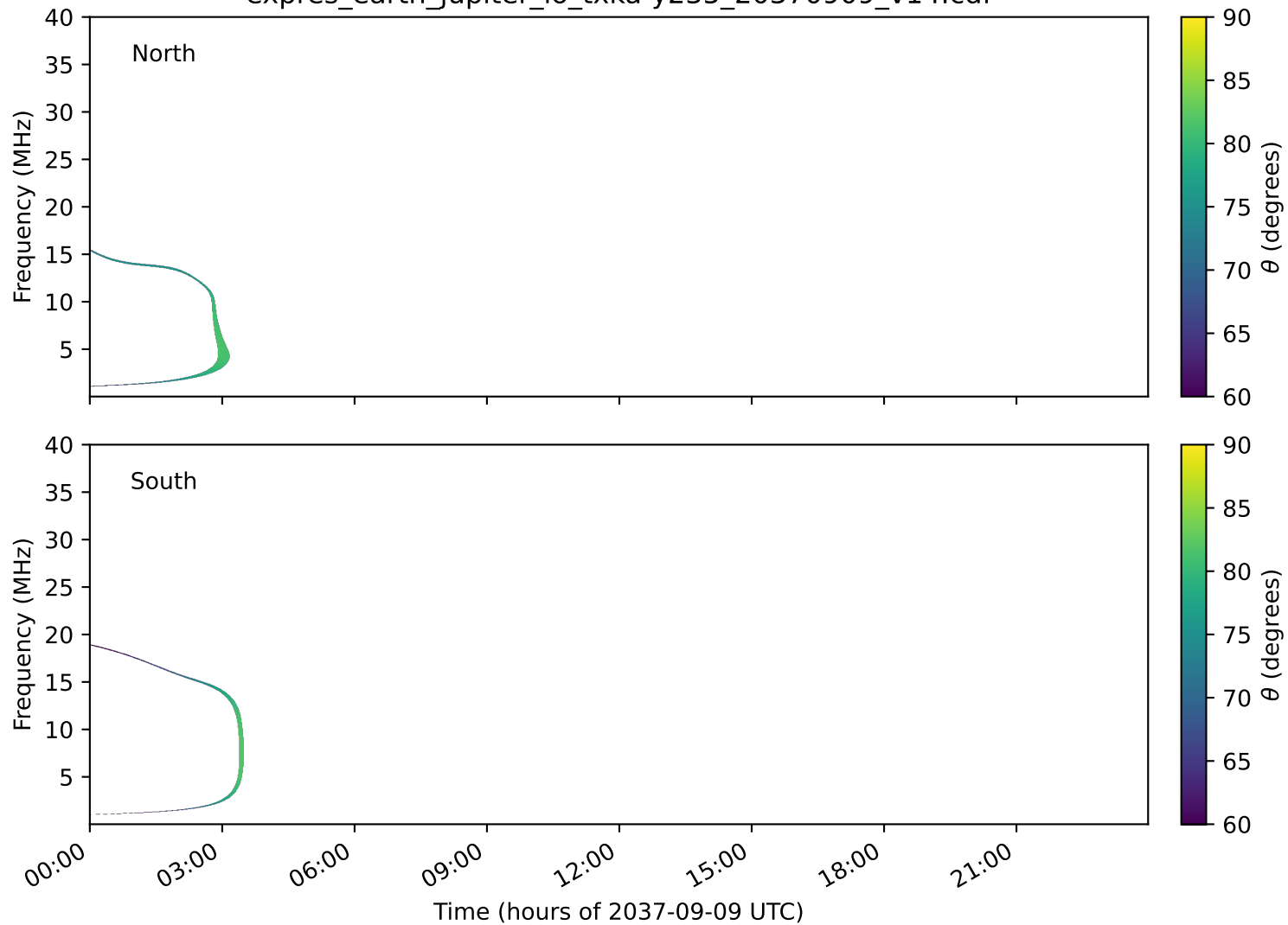
expres_earth_jupiter_io_txka-y235_20370909_v14.cdf
