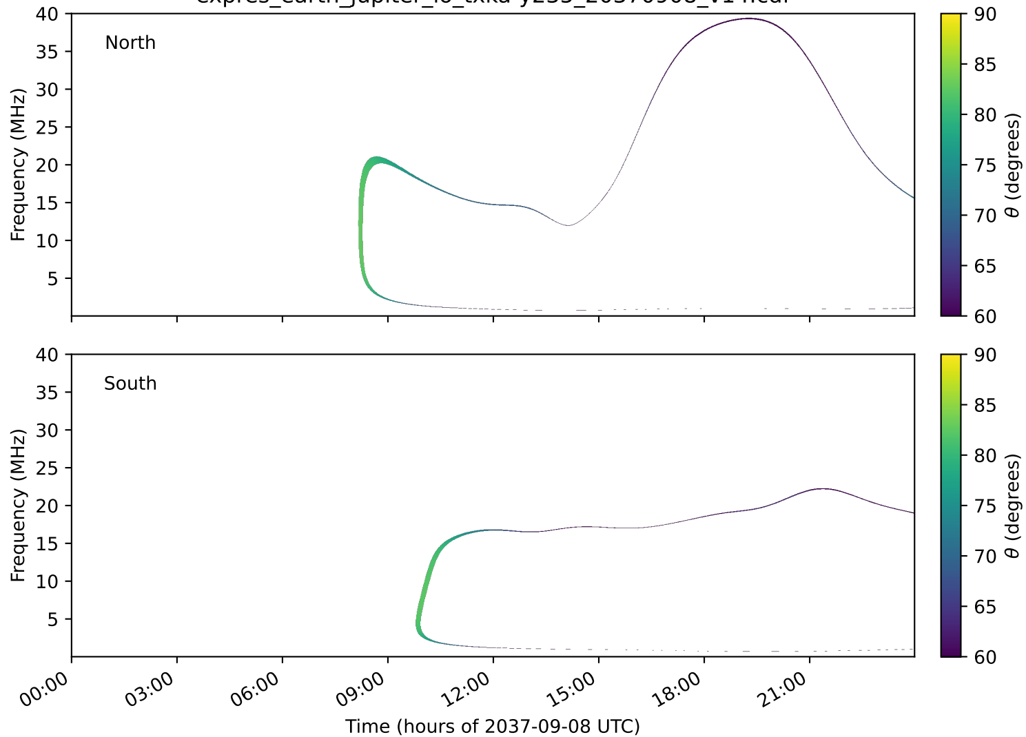
expres_earth_jupiter_io_txka-y235_20370908_v14.cdf
