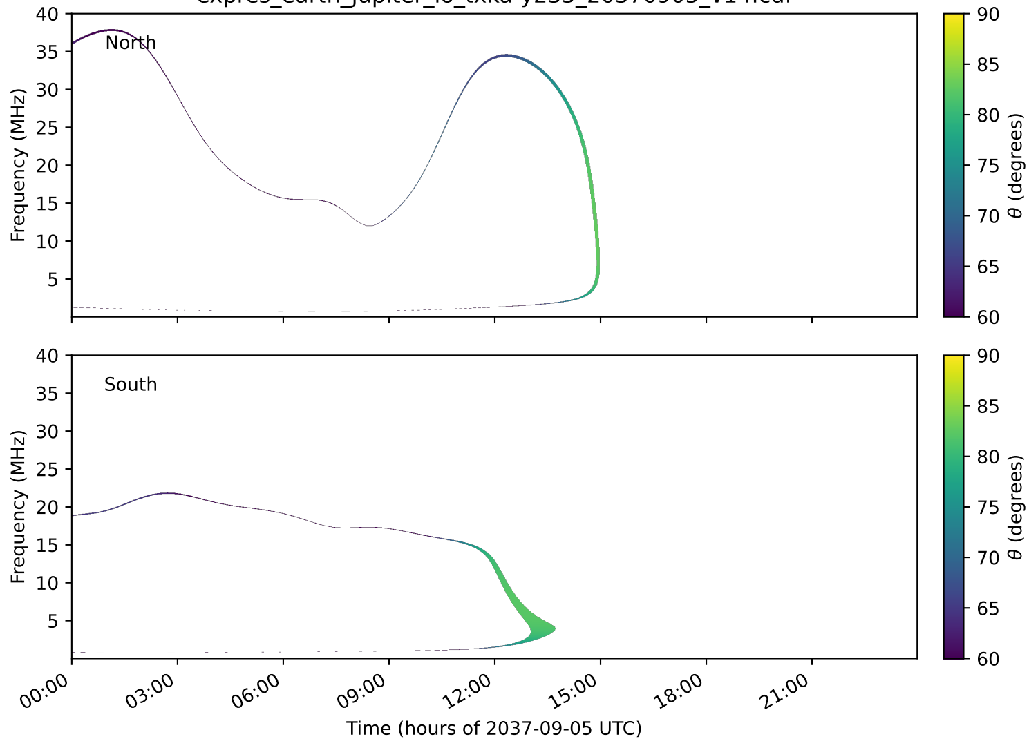
expres_earth_jupiter_io_txka-y235_20370905_v14.cdf
