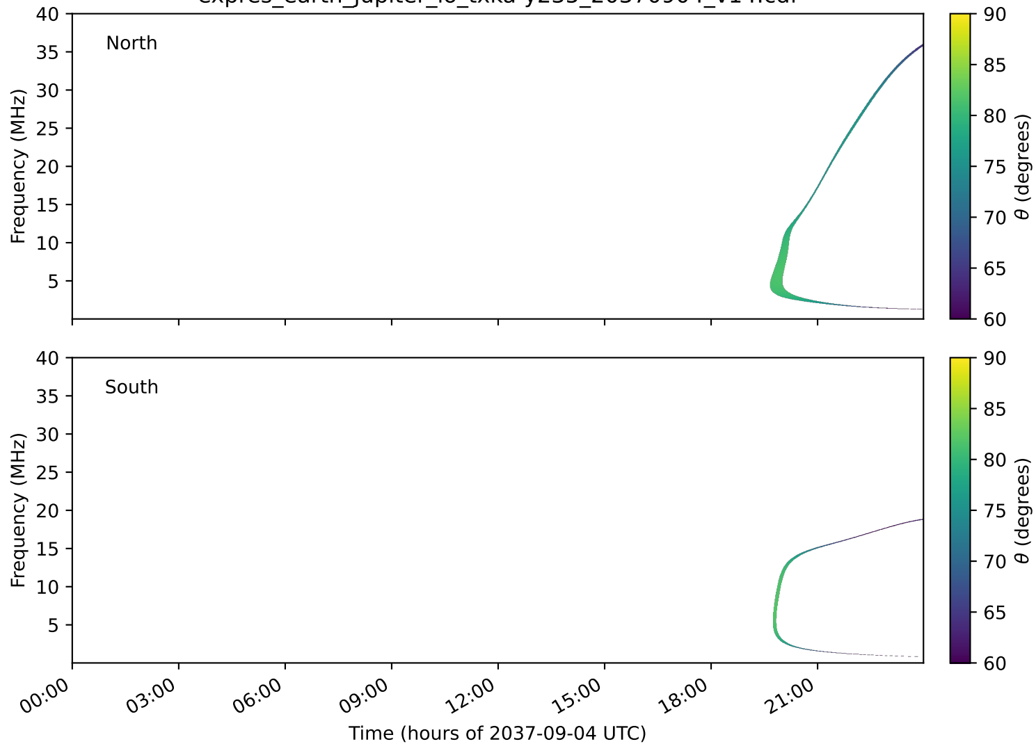
expres_earth_jupiter_io_txka-y235_20370904_v14.cdf
