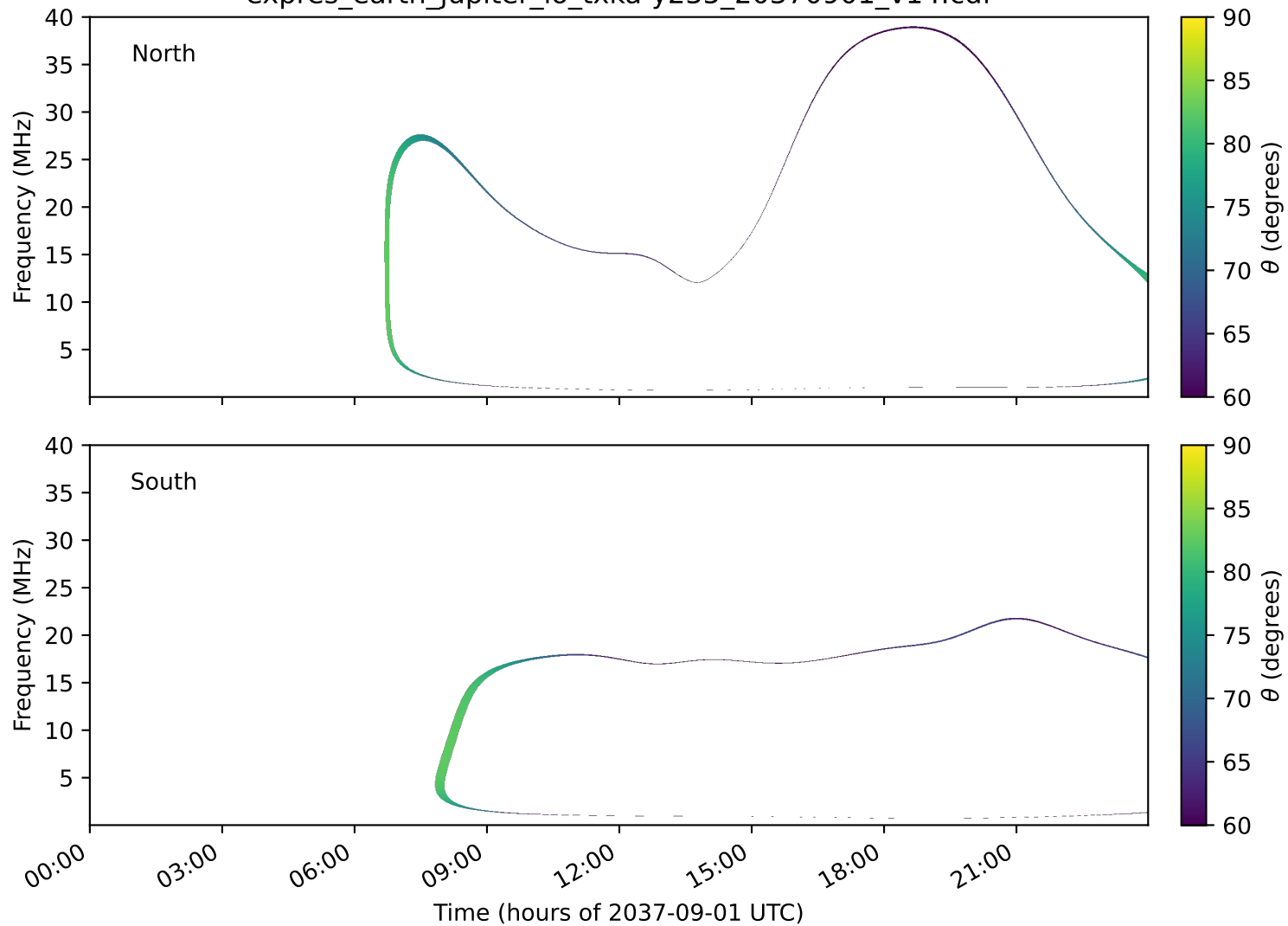
expres_earth_jupiter_io_txka-y235_20370901_v14.cdf
