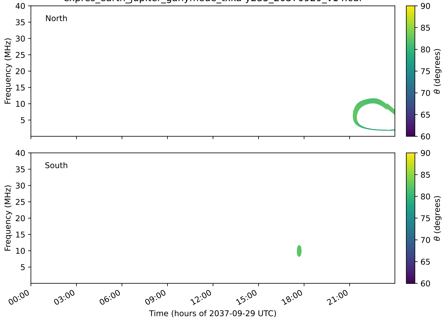
expres_earth_jupiter_ganymede_txka-y235_20370929_v14.cdf
