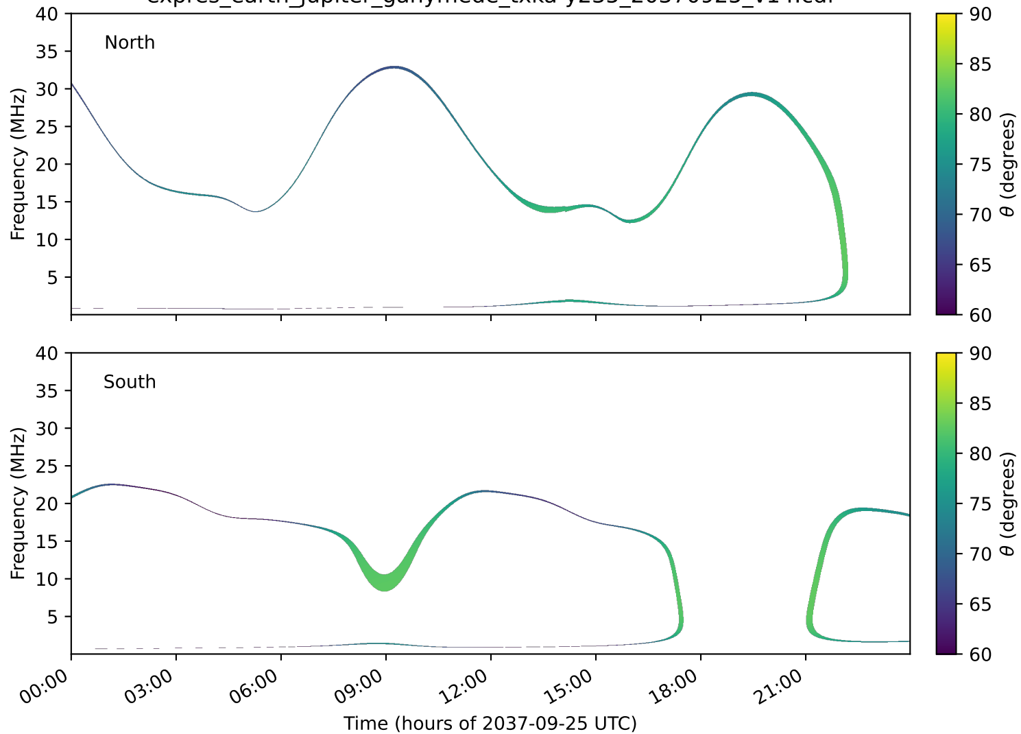
expres_earth_jupiter_ganymede_txka-y235_20370925_v14.cdf
