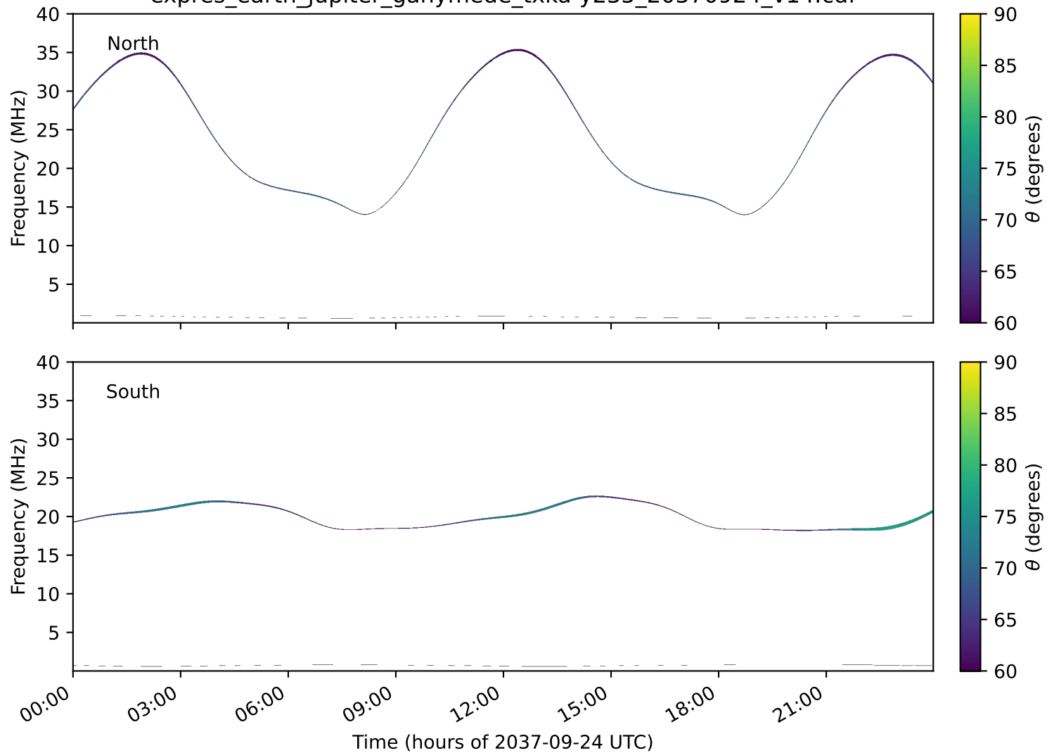
expres_earth_jupiter_ganymede_txka-y235_20370924_v14.cdf
