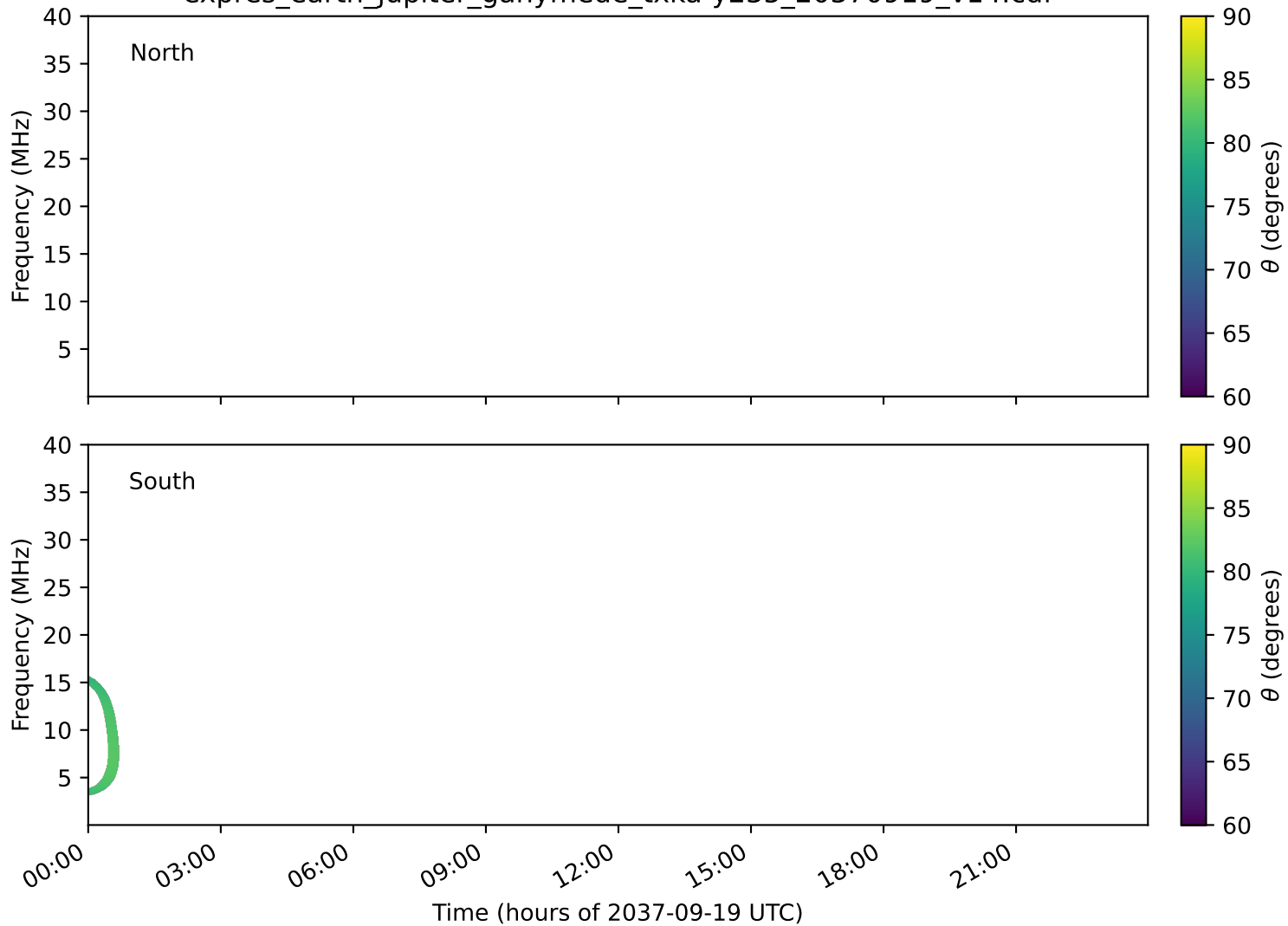
expres_earth_jupiter_ganymede_txka-y235_20370919_v14.cdf
