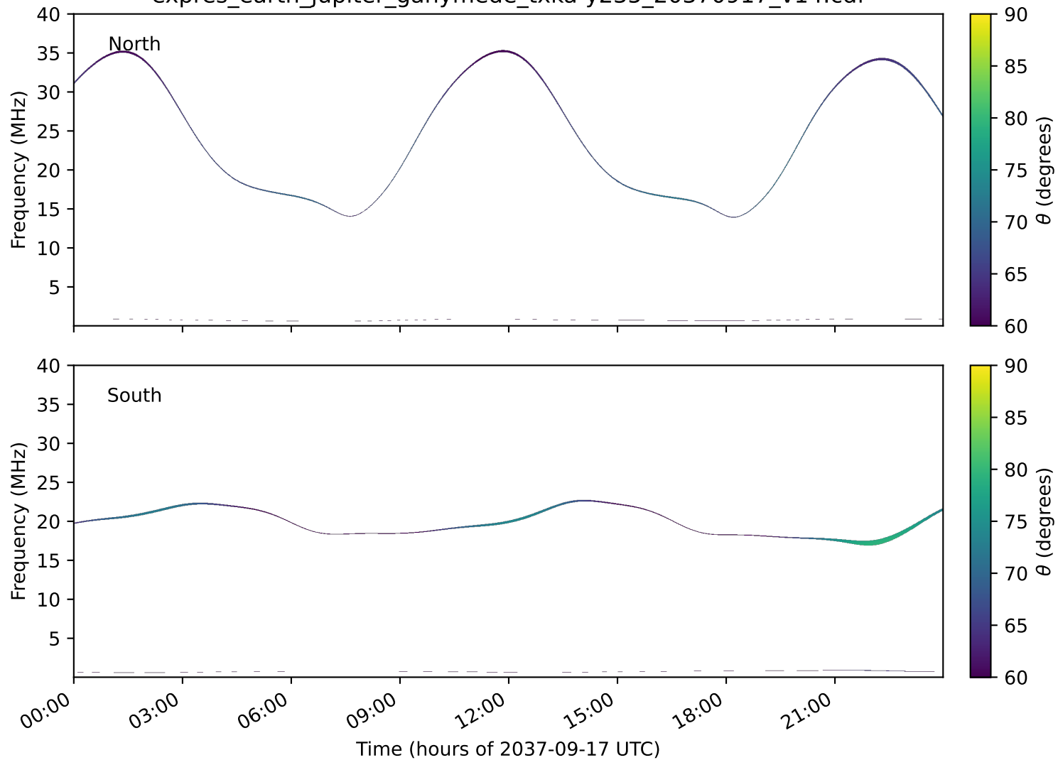
expres_earth_jupiter_ganymede_txka-y235_20370917_v14.cdf
