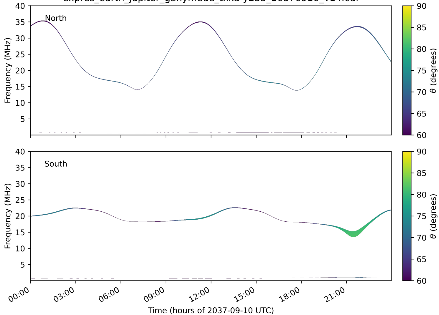
expres_earth_jupiter_ganymede_txka-y235_20370910_v14.cdf
