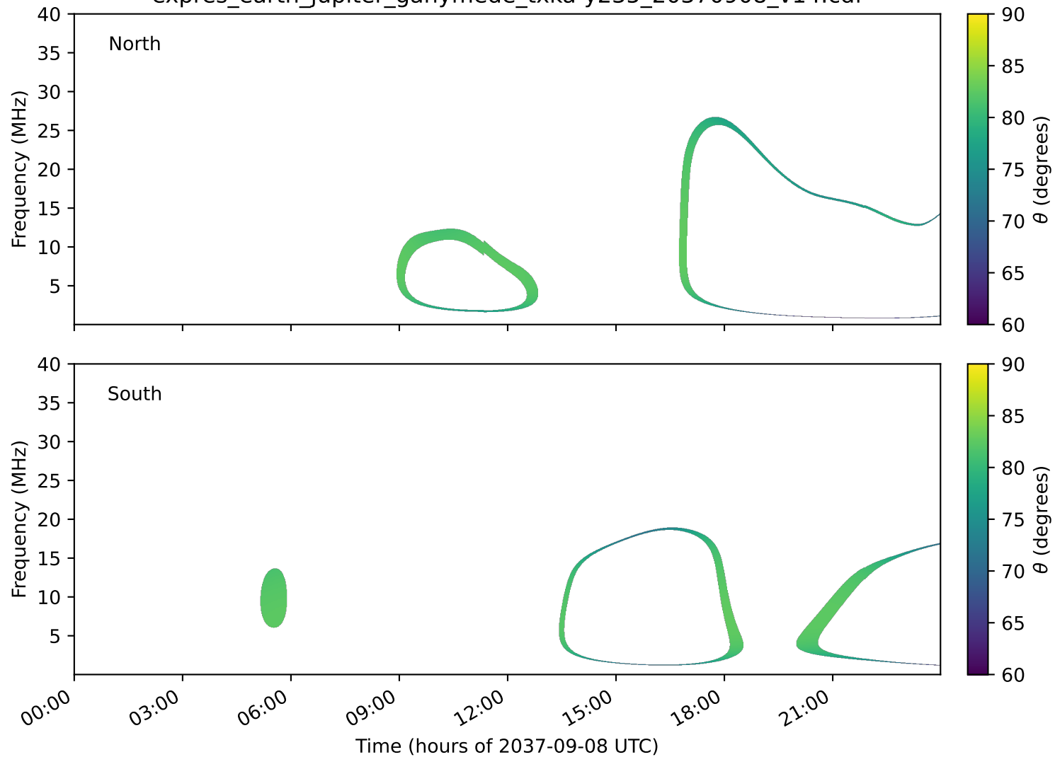
expres_earth_jupiter_ganymede_txka-y235_20370908_v14.cdf
